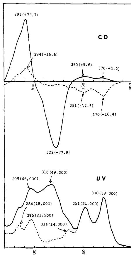
Figure 1. Measurements in \text{CHCl}_3 , UV and CD curves of dihydrodiol 2a (---) and its dma-dibenzoate 5 (—). Only regions above 270 nm are shown due to difficulty in CD measurements. The absorption, centered at 295 and 351 nm, is due to the longitudinal and transverse transitions of the dihydrobenzo[ a ]pyrene moiety, respectively.
